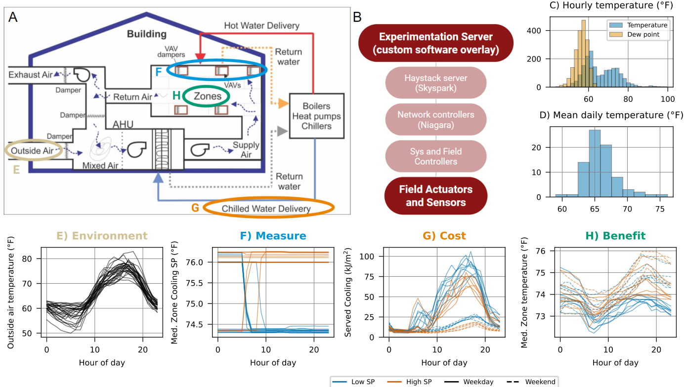
Figure 1: Experiment testbed and illustration of experimentation protocols. (A) Building schematic. (B) Software overlay. (C-D) Histograms for hourly temperature and daily averages measured at the campus weather station. (E-H) Daily profiles for key variables in OFF-2 where mean daily outside air temperatures are between 65°F and 67°F (11 days of high set points and 14 days of low set points). A dew point below 60°F is typically associated with dry conditions.
