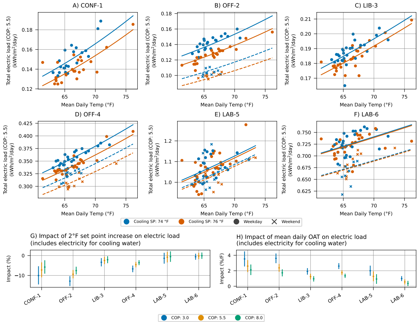
Figure 3: Experiment results: electricity loads (including for cooling water). (a) Daily electricity as a function of mean daily temperatures of the cooling set points. Empirical data collected during the summer of 2021 and log model from equation 1. (b) Measured effect of OAT and set point change on electricity. To estimate the electricity required for cooling water, different assumptions are made for chiller Coefficient Of Performance (COP). Numerical results for a COP of 5.5 are reported in Table S4.
