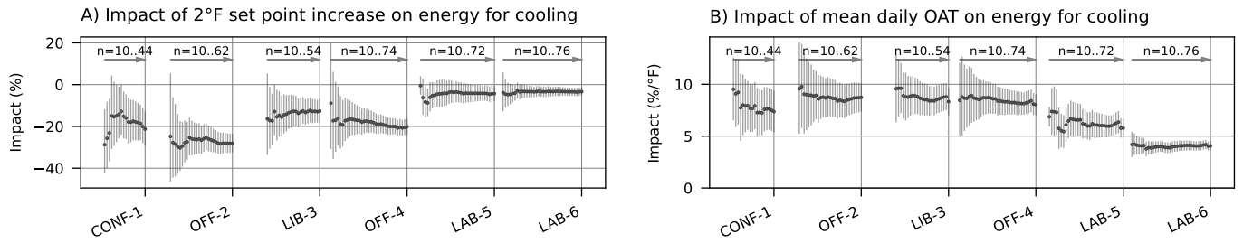
Figure 5: Collecting a growing number of observations gradually improves parameter estimates. Measured effect of set point change and OAT on energy for cooling using the model in Section 4.1. The dots represent the average estimates and the vertical bars show the 95% confidence intervals. The number of observations (n) is reported for each building, e.g. 10 to 44 observations are used for CONF-1.
