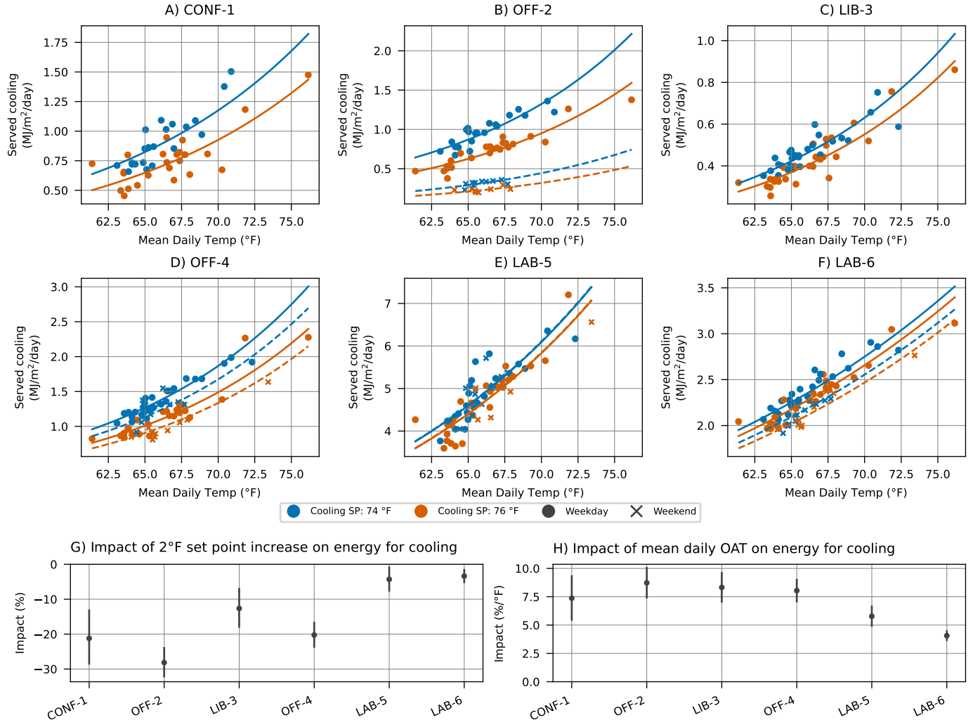
Figure 2: Experiment results: energy for cooling. A-F) Daily energy for cooling increases with mean daily temperatures and decreases when the cooling set points are increased. Empirical data collected during the summer of 2021 and log model from equation 1. G-H) Measured effect of OAT and set point change on energy for cooling. Additional numerical results are reported in Table S2 and data in different units are shown in Figures 1 and 2. Model structure and predictors are discussed in Section 5.
