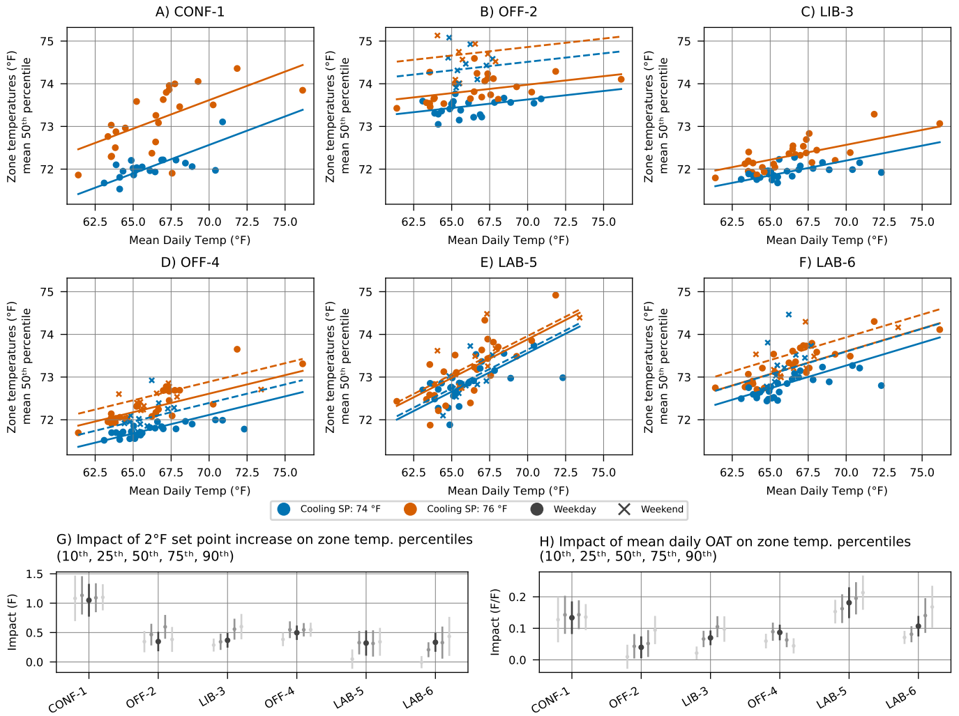
Figure 4: Experiment results: room temperatures. (a) The 8am-8pm average for the 50 th percentile of room temperatures increases with mean daily OAT and as the cooling set points are increased. Numerical results are reported in Table S5.
